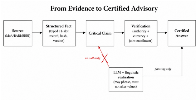
Figure 1: Agricultural Claim Authority and Joint Entailment Model. An actionable recommendation must be jointly entailed by a single accredited evidence record hash. Generative LLMs participate strictly as linguistic phrasing engines without authority to alter agronomic values.
